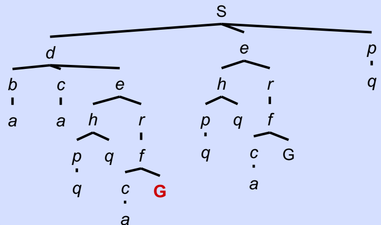
Search Tree
