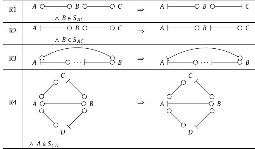
Figure 10: Orientation rules in Algorithms 4 and 5: Rules R1-R4 (Peña, 2012)
