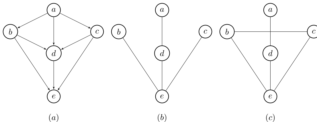
Figure 8: Order-dependent skeleton of the PC-LIKE algorithm. (a) The DAG G , (b) the skeleton returned by Algorithm 4 with order_1(V) , (c) the skeleton returned by Algorithm 4 with order_2(V) .
